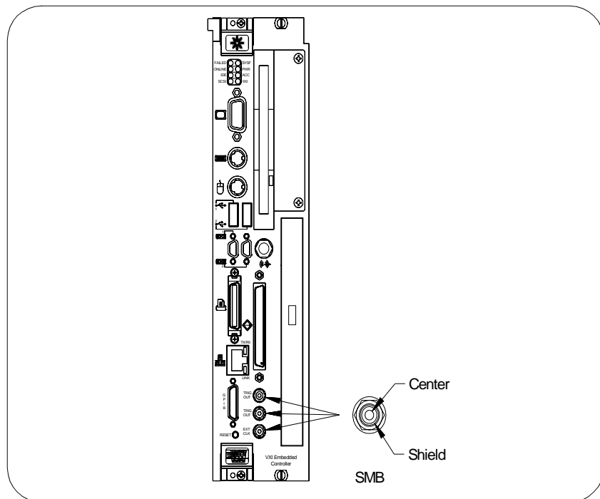
Figure E-10. SMB Connectors Location and Pinout
