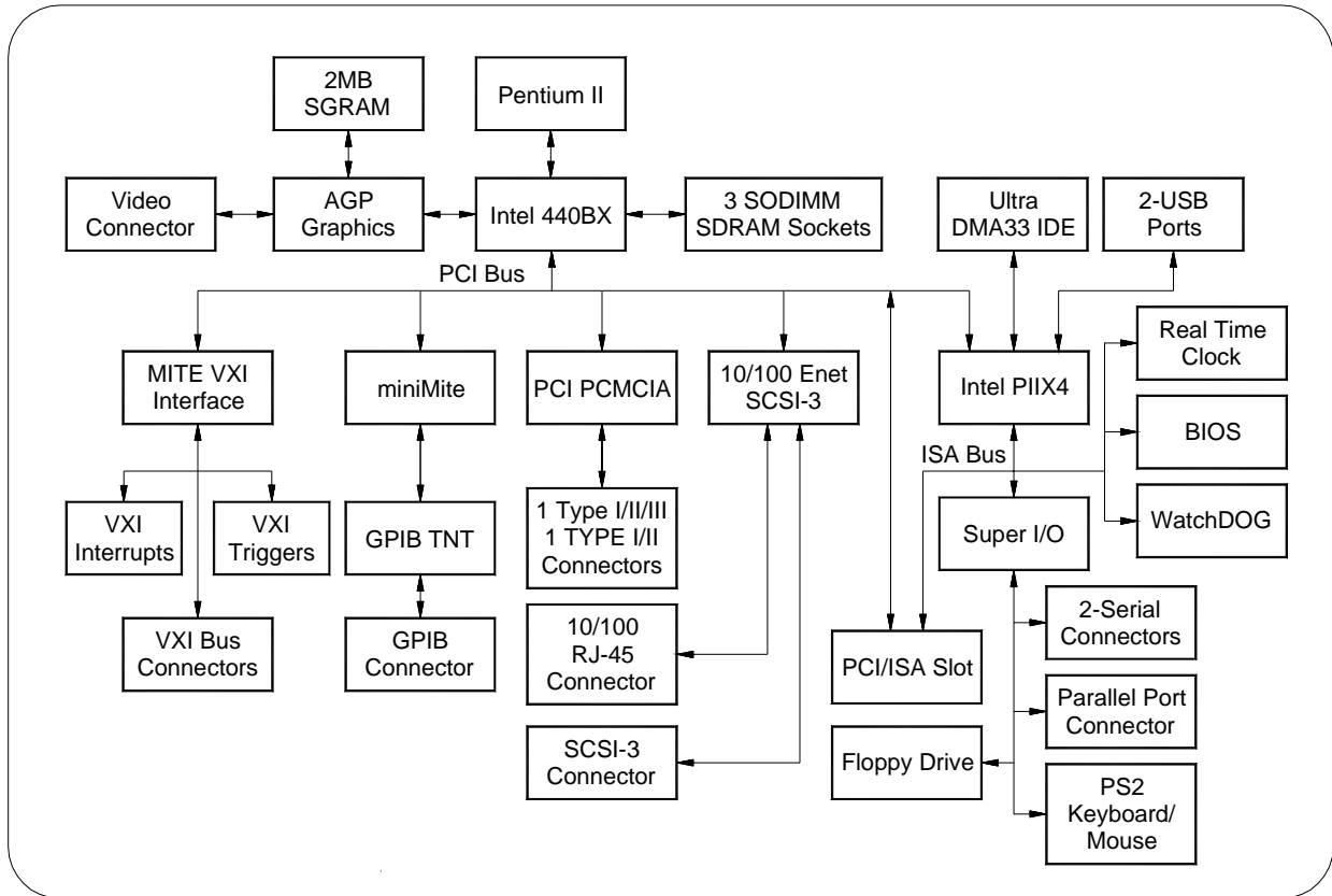
Figure 4-2. E9850A Functional Block Diagram
