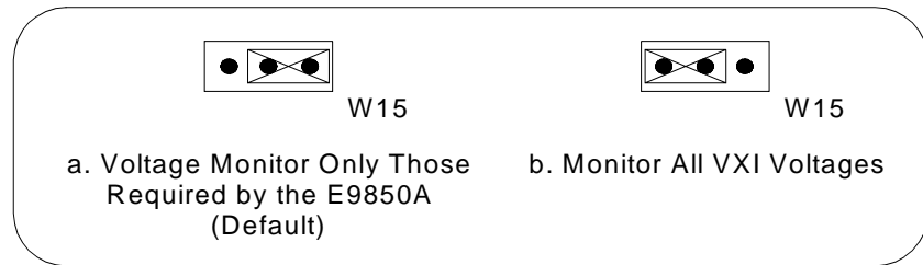
Figure 5-11. Voltage Monitor Settings
