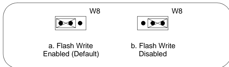
Figure 5-9. Flash Protection Jumper Settings
