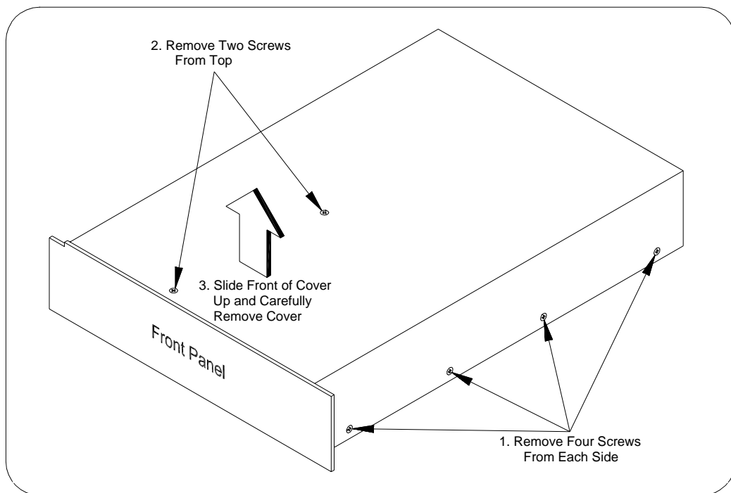
Figure 6-2. Removing the E9850A Cover
