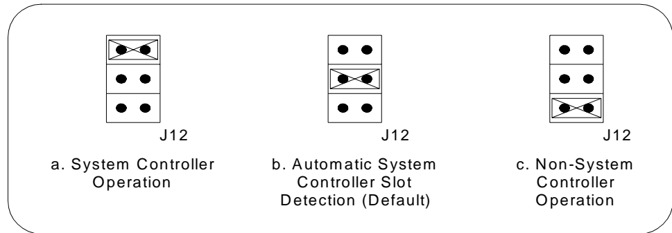
Figure 5-2. System Controller Operation Switch Settings
