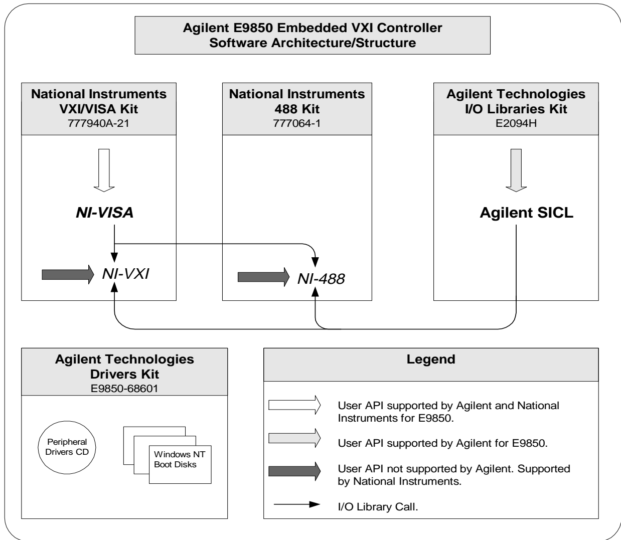
Figure 1-2. E9850A Software Architecture/Support
