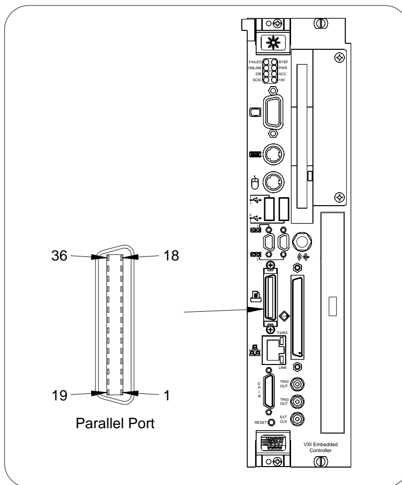
Figure E-6. Parallel Port Connector Location and Pinouts
