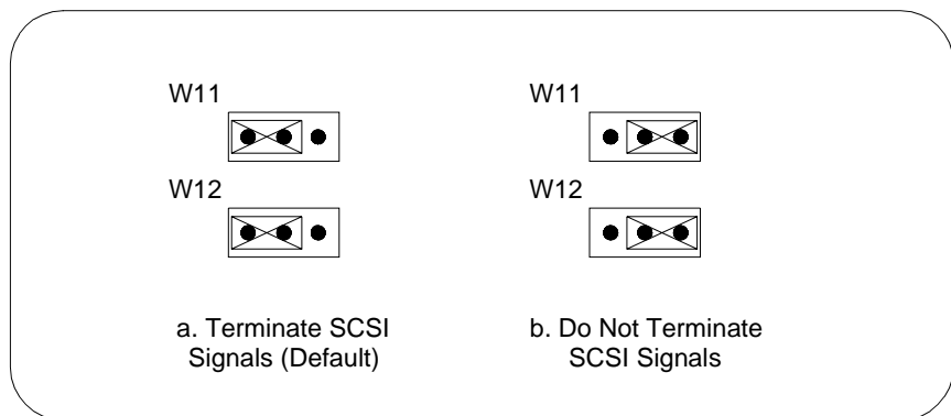
Figure 5-5. SCSI Termination
