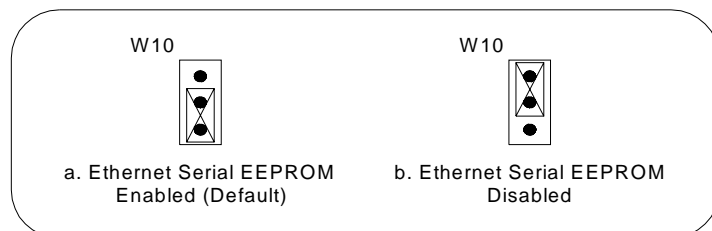
Figure 5-10. Ethernet Serial EEPROM Settings
