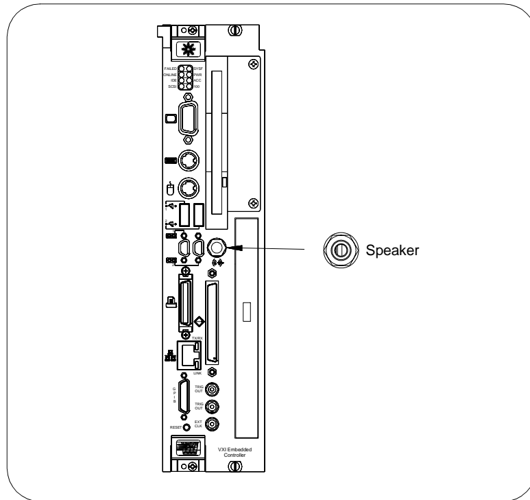
Figure E-4. Speaker Connection Location
