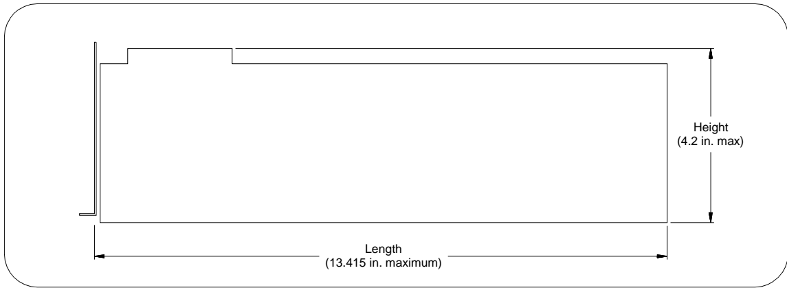
Figure 6-4. I/O Board Dimensions for E9850A Expansion Slot
