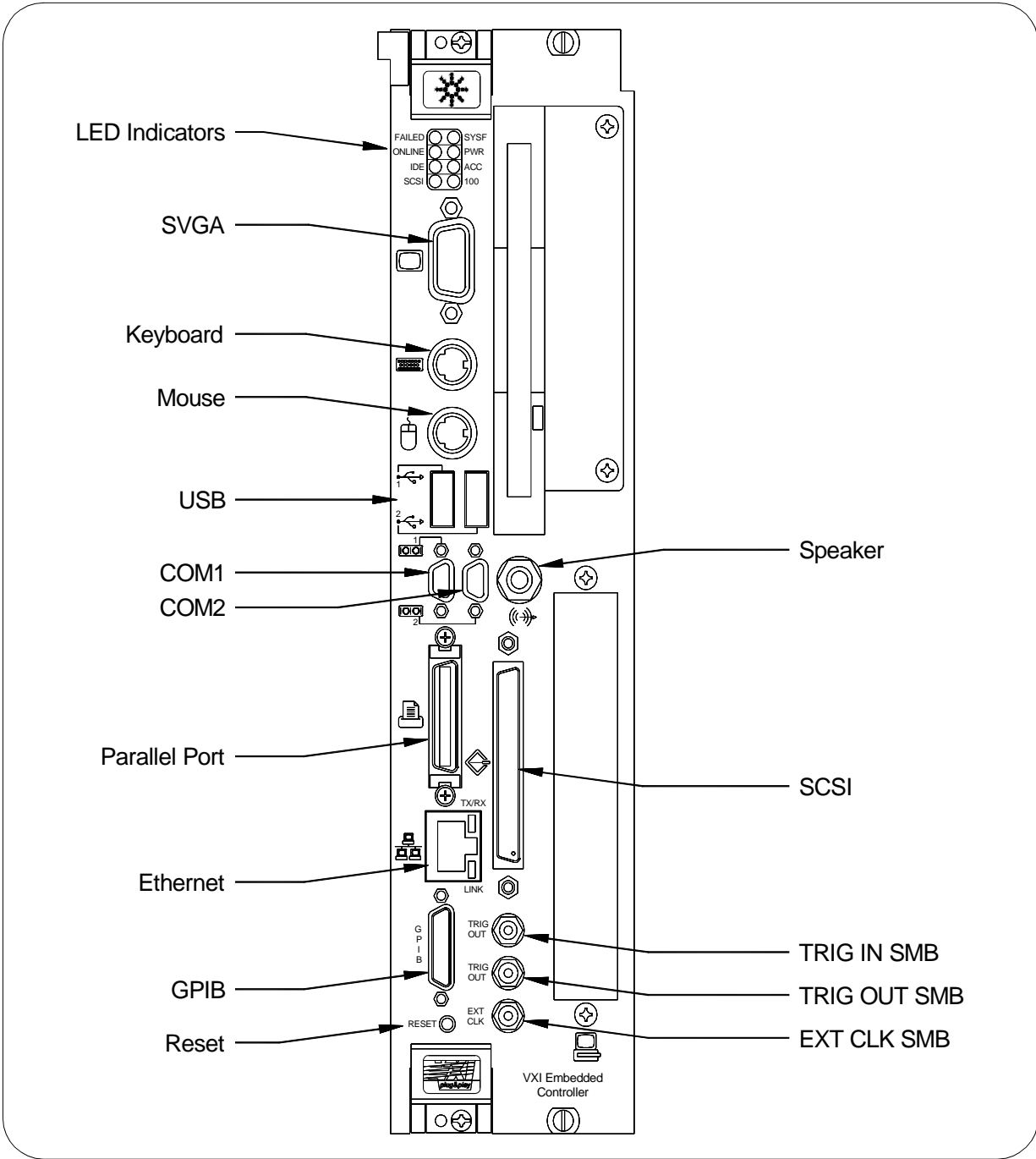
Figure 4-1. E9850A Front Panel Features
