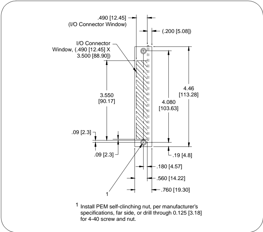
Figure 6-7. Front View of ISA Board Front Panel Bracket
