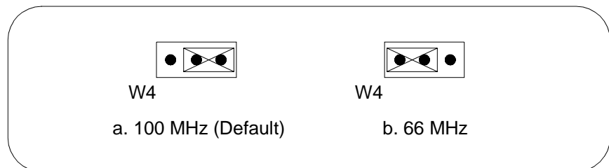
Figure 5-7. CPU Bus Speed Configuration
