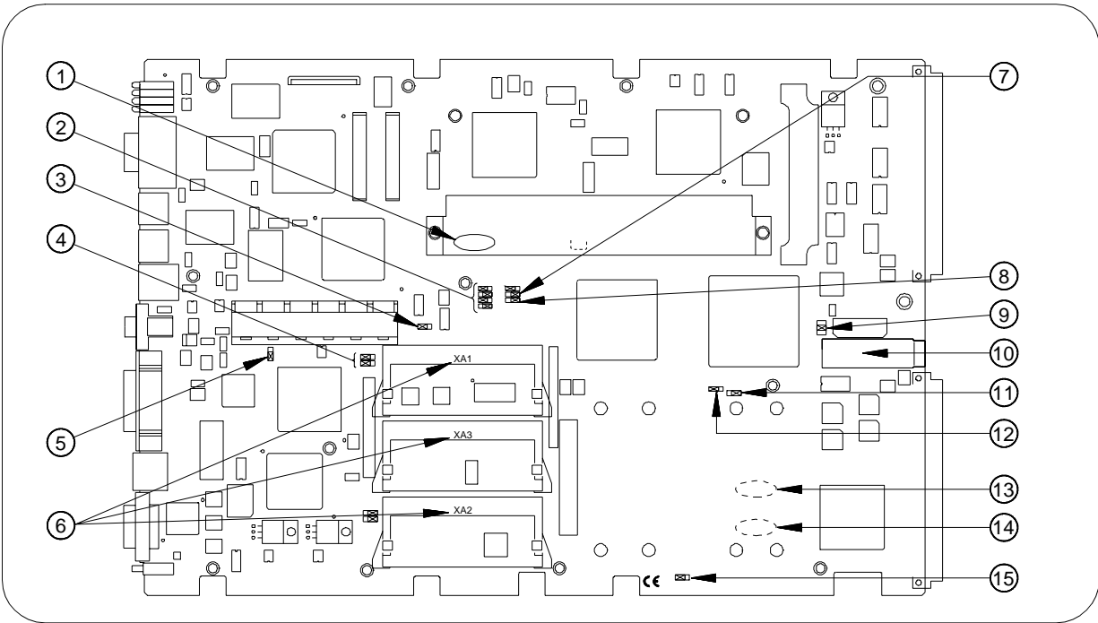
Figure 5-1. E9850A Switch/Jumper Locations
