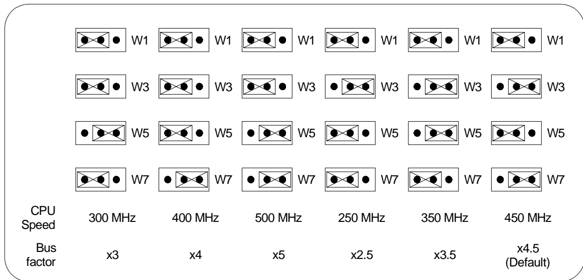
Figure 5-8. CPU Bus Factor Jumper Settings
